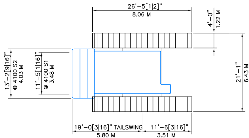
OUTLINE DIMENSIONS
