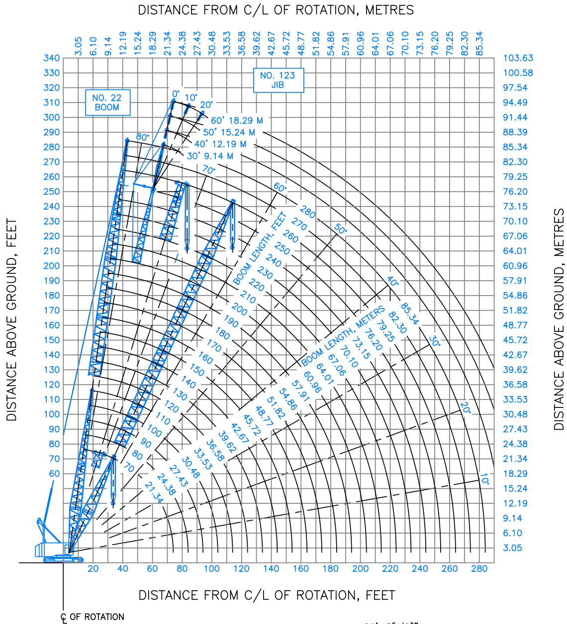
RANGE DIAGRAM
